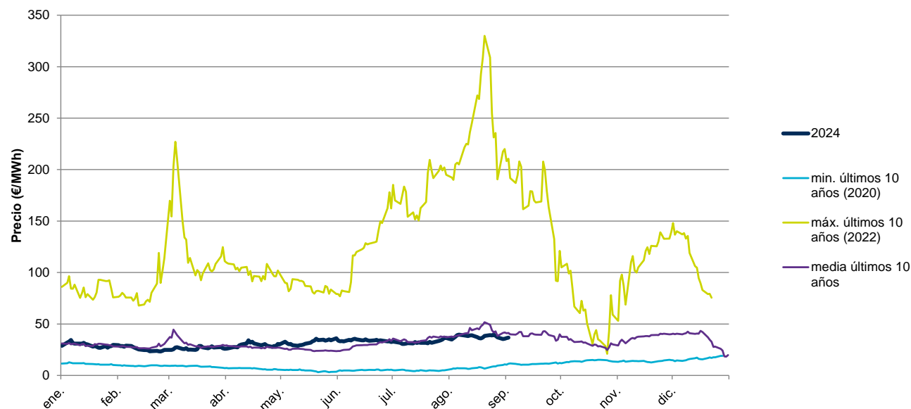
TTF Day Ahead - 2024
